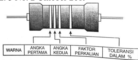
Gambar 4. Garis warna resistor (Wikipedia.com)
