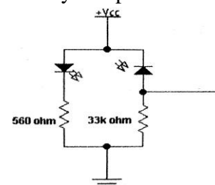
Gambar 15. Rangkaian sensor (Wikipedia.com)
