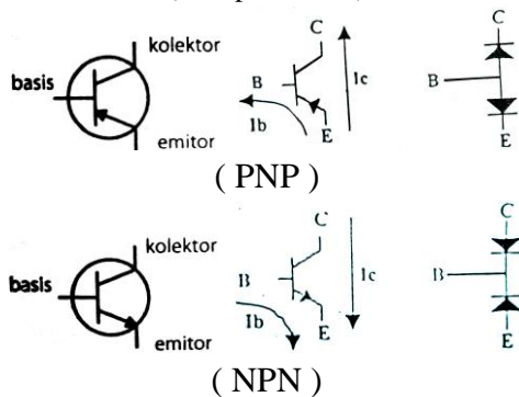
Gambar 6. Simbol transistor (Wikipedia.com)
