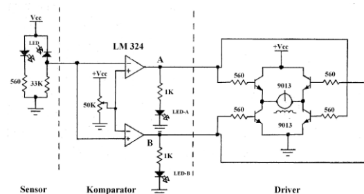
Gambar 14. Rangkaian Line Follower (Wikipedia.com)
