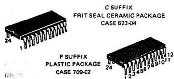
Gambar 11. IC (Wikipedia.com)
