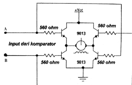
Gambar 19. Rangkaian driver (Wikipedia.com)
