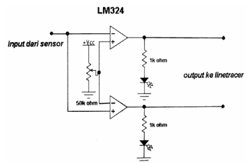
Gambar 18. Rangkaian komparator (Wikipedia.com)
